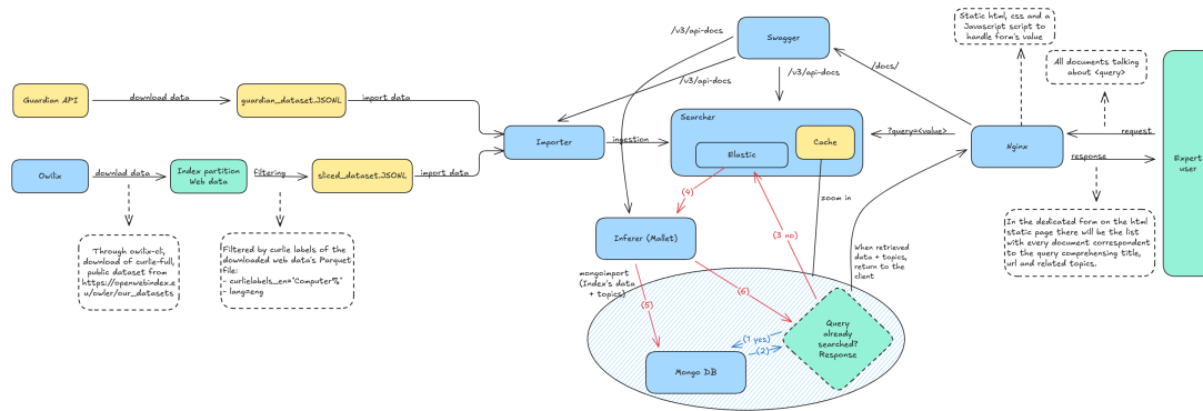
Figure 1: System pipeline overview. Blue elements represent services instantiated in separate Docker containers; yellow elements represent auxiliary components such as scripts or files; green blocks represent logical groupings introduced for clarity.
