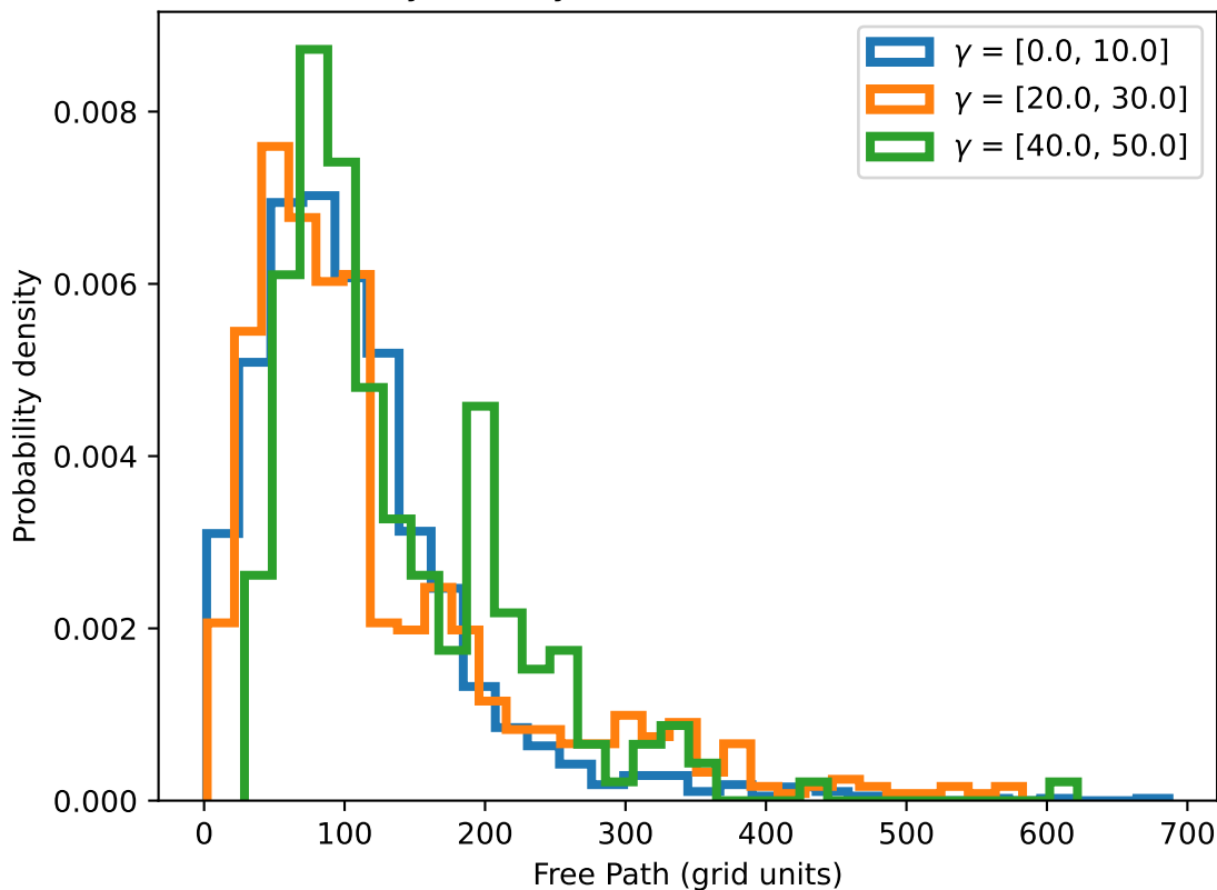
Probability Density of Free Paths for 1000 Particles
