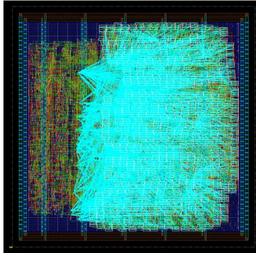
Figure 5: The register file selected across the die. All 992 flip-flops matching datapath/registers_RF_reg, which is 31 architectural registers of 32 bits each, x0 costing nothing because it is hardwired to zero.
