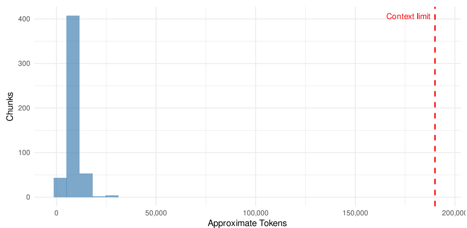
Figure 1: Approximate token count per chunk (C2 input)
