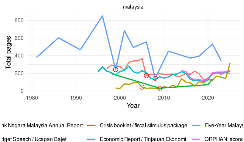
Figure 6: Pages per year and body; red circles mark sudden drops ( >50\% YoY)
