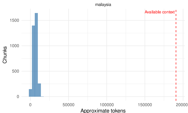
Figure 7: Chunk token distribution with available-context reference line
