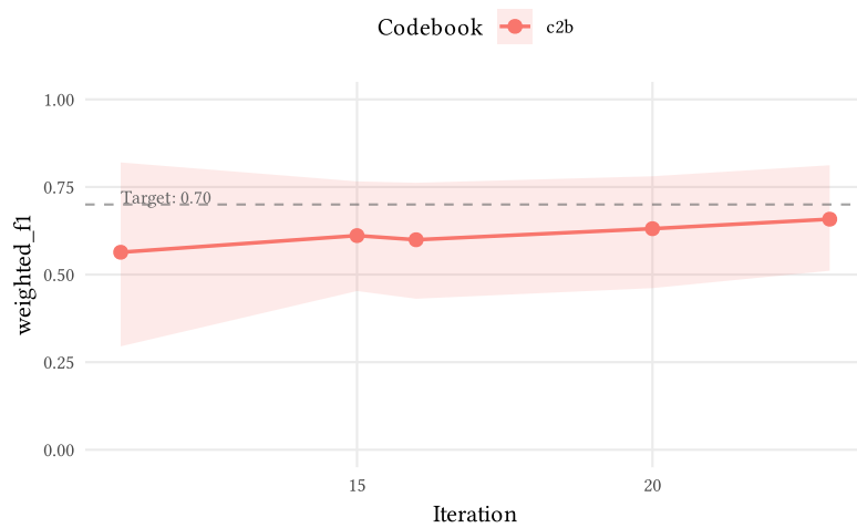
Figure 3: C2b weighted F1 across formal (Claude) iterations
