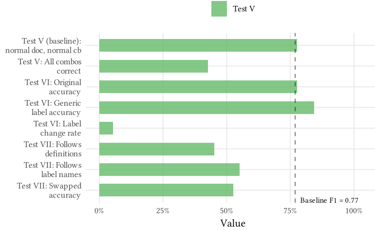
Figure 5: C1 S3 behavioral tests (latest formal run)
