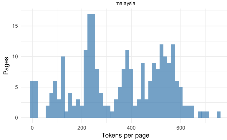
Figure 4: Token distribution per page across the sampled documents
