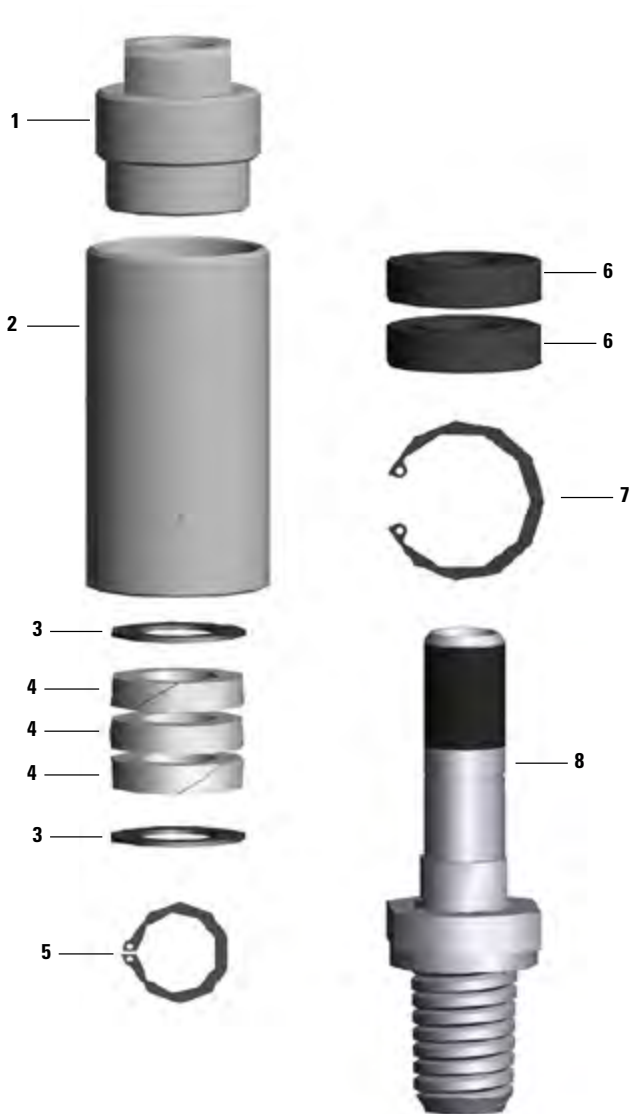
AWJ Teflon & Ceramic Water Swivel
