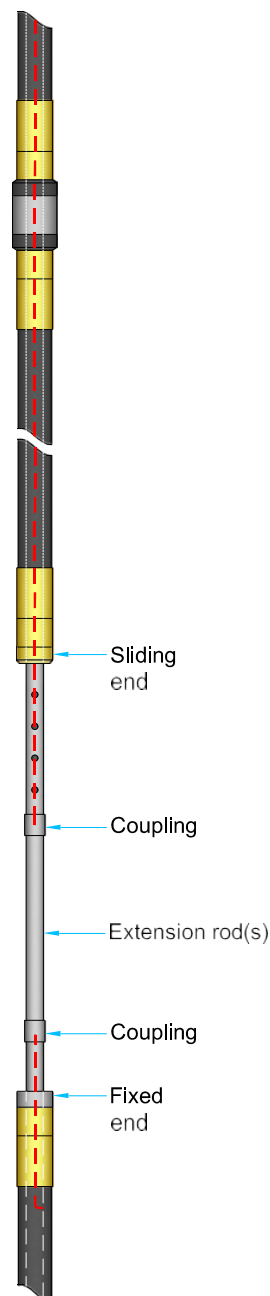
TYPE "C" TYPE "B" + EXTENSION ROD(S)
