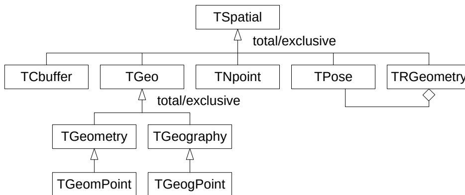
Figure 7.1: Hierarchy of spatiotemporal types in MobilityDB.
