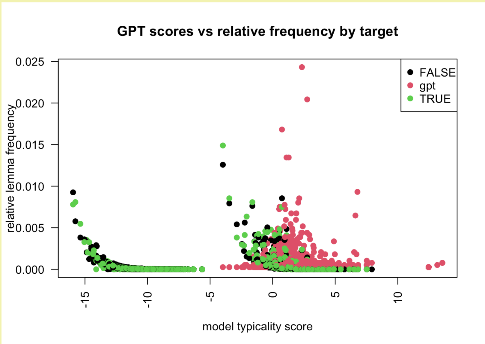
Figure 3: model typical vocab distribution
