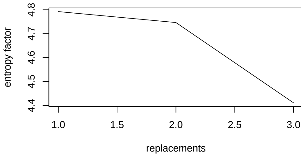
Figure 1: entropy plot
