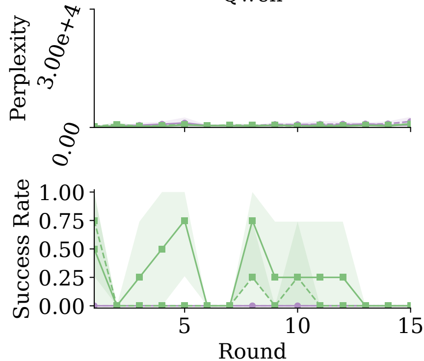
Qwen
