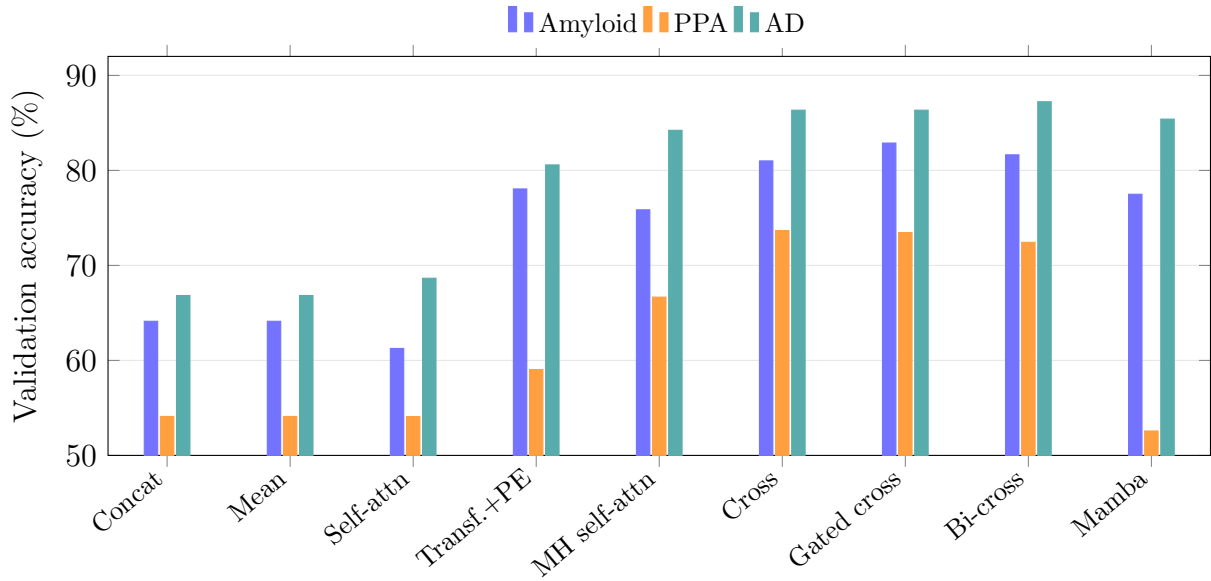
Figure 11: Validation accuracy of the fusion families on the three tasks (values from Table 8). The cross-attention family leads on every task, while Mamba’s drop to chance on PPA stands out as the clearest outlier. Abbreviations: Concat = concatenation, Mean = element-wise mean (both non-sequential baselines); Self-attn = self-attention, MH self-attn = multi-head self-attention, Transf.+PE = transformer with positional encoding; Cross = cross-attention, Gated cross = gated cross-attention, Bi-cross = bidirectional cross-attention; Mamba = selective state-space fusion.
