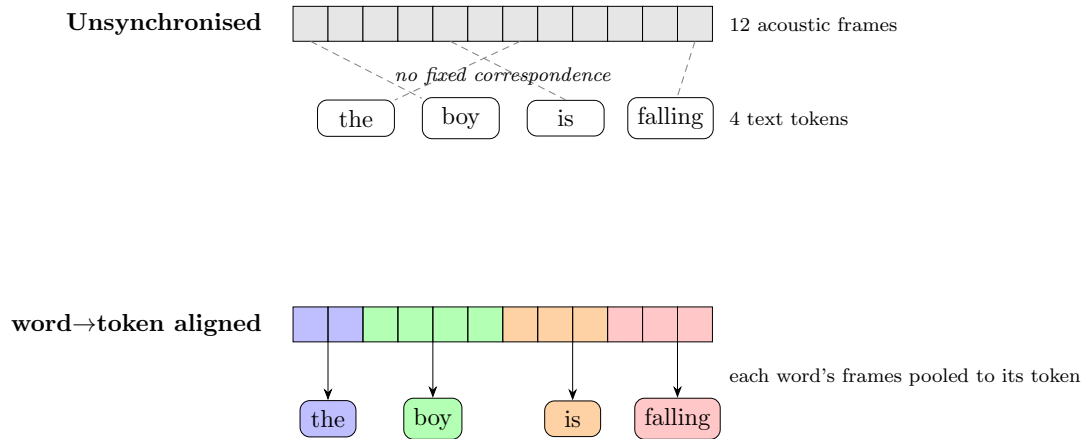
Figure 3: Cross-modal alignment between acoustic frames and text tokens, comparing unsynchronised input (top), where the two streams have no fixed correspondence, with word-to-token aligned input (bottom), where the frames spanned by each spoken word are pooled and attached to that word’s token.
