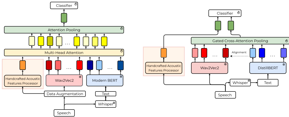
Figure 9: Architectural comparison of the two primitive stacks. The left panel shows the Double Multi-Head Attention Module (DMHAM) system; the right panel shows the CogniAligned framework. The two are used throughout this thesis as independent implementations, so trends that reproduce across them are read as properties of the technique rather than of one codebase.
