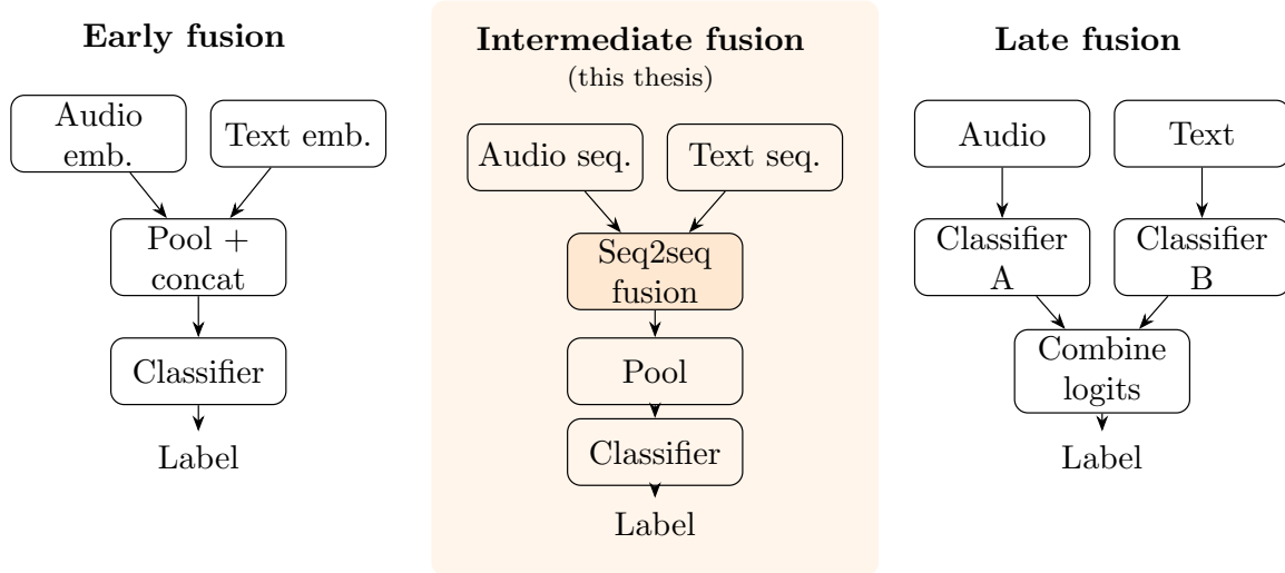
Figure 2: The three multimodal fusion paradigms. Early fusion pools and concatenates the modality embeddings into one vector before a single classifier; late fusion trains a classifier per modality and combines their outputs; intermediate fusion, the paradigm used in this thesis, processes both sequences jointly through a sequence-to-sequence module before pooling and classification.
