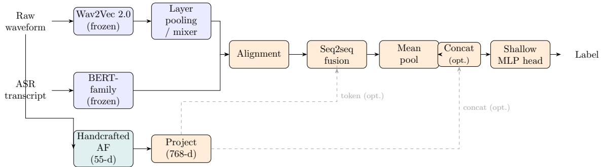
Figure 8: End-to-end architecture used in this thesis: frozen Wav2Vec 2.0 and BERT-family encoders (blue) produce acoustic and textual sequences, which are placed on a common index by the alignment step, combined by the trainable sequence-to-sequence fusion module (orange), and mapped to a task label by a shallow head. A parallel branch extracts 55-dimensional handcrafted acoustic descriptors from the waveform (teal), projects them to the model width, and joins the pipeline either as an extra fusion token or by concatenation after pooling (dashed, optional). Blue blocks are frozen, orange blocks are trained.
