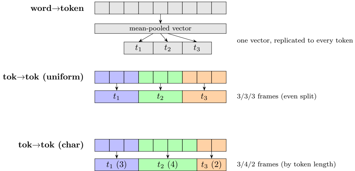
Figure 6: Audio-text alignment schemes compared in this thesis, for one spoken word whose nine acoustic frames are split across three subword tokens of character lengths 3/4/2. The CogniAlign word-to-token baseline mean-pools all frames into a single vector and replicates it to every token; the proposed uniform scheme divides the frames evenly across the tokens; the proposed proportional (char) scheme allocates frames in proportion to each token’s character length.
