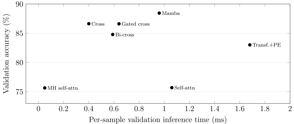
Figure 11: Validation accuracy against per-sample inference time for the fusion families in the precomputed-embedding (CogniAligned) pipeline (fusion study, ADReSSo).
