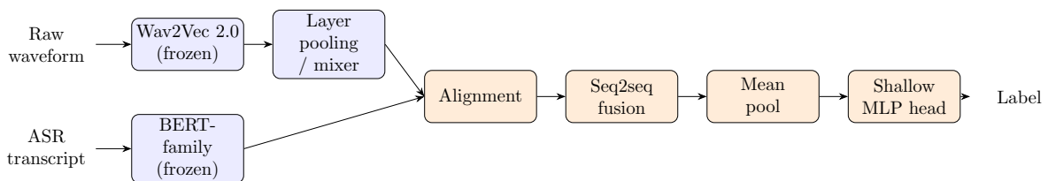
Figure 5: End-to-end architecture used in this thesis: frozen Wav2Vec 2.0 and BERT-family encoders (blue) produce acoustic and textual sequences, which are placed on a common index by the alignment step, combined by the trainable sequence-to-sequence fusion module (orange), and mapped to a task label by a shallow head. Blue blocks are frozen, orange blocks are trained.
