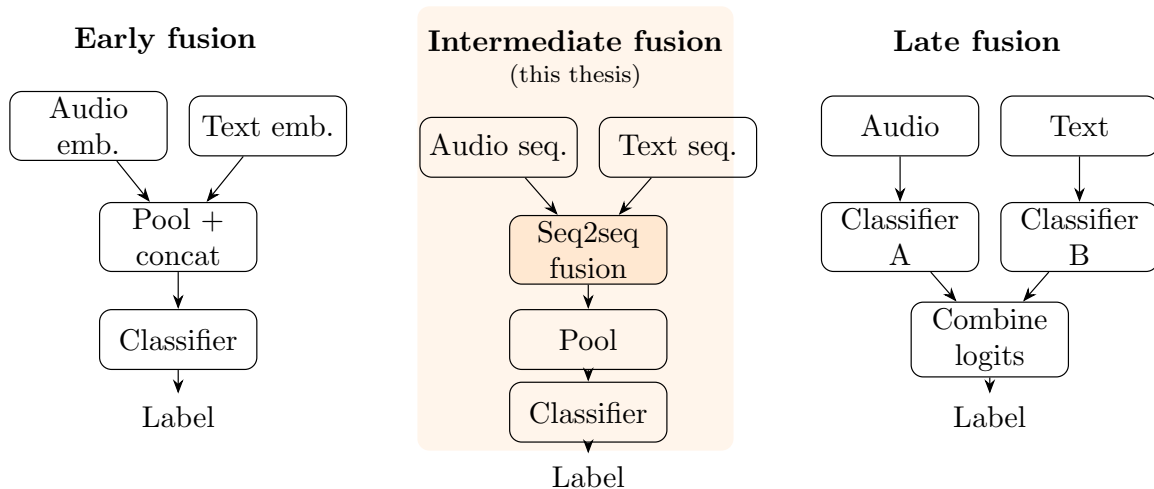
Figure 3: The three multimodal fusion paradigms. Early fusion pools and concatenates the modality embeddings into one vector before a single classifier; late fusion trains a classifier per modality and combines their outputs; intermediate fusion, the paradigm used in this thesis, processes both sequences jointly through a sequence-to-sequence module before pooling and classification.
