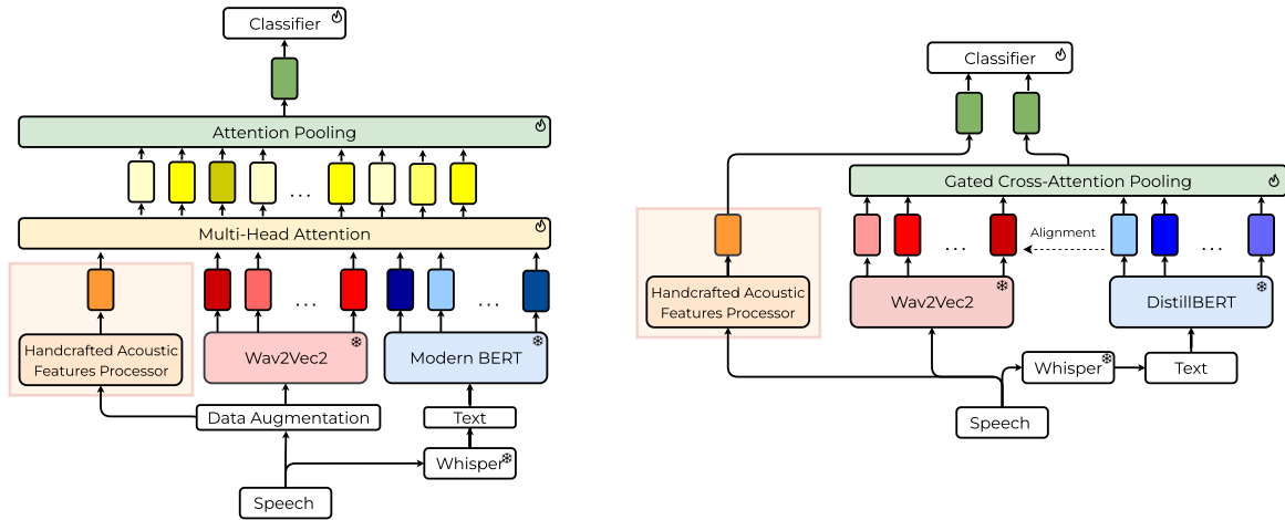
Figure 4: Architectural comparison of the two multimodal frameworks this thesis builds on. The left panel shows the Double Multi-Head Attention Multimodal (DMHAM) system; the right panel shows the CogniAlign framework. They share a two-stream skeleton but differ in their encoders, ASR, and alignment: CogniAlign aligns acoustic frames to subword tokens, whereas DMHAM fuses segment-level representations.
