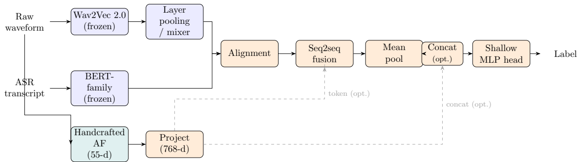
Figure 9: End-to-end architecture used in this thesis: frozen Wav2Vec 2.0 and BERT-family encoders (blue) produce acoustic and textual sequences, which are placed on a common index by the alignment step, combined by the trainable sequence-to-sequence fusion module (orange), and mapped to a task label by a shallow head. A parallel branch extracts 55-dimensional handcrafted acoustic descriptors from the waveform (teal), projects them to the model width, and joins the pipeline either as an extra fusion token or by concatenation after pooling (dashed, optional). Blue blocks are frozen, orange blocks are trained.
