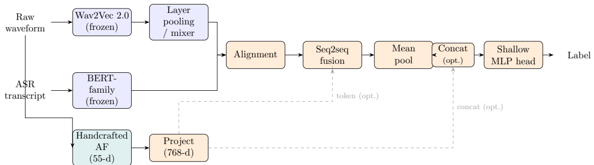
Figure 9: End-to-end architecture used in this thesis: frozen Wav2Vec 2.0 and BERT-family encoders (blue) produce acoustic and textual sequences, which are placed on a common index by the alignment step, combined by the trainable sequence-to-sequence fusion module (orange), and mapped to a task label by a shallow head. A parallel branch extracts 55-dimensional handcrafted acoustic descriptors from the waveform (teal), projects them to the model width, and joins the pipeline either as an extra fusion token or by concatenation after pooling (dashed, optional). Blue blocks are frozen, orange blocks are trained.
