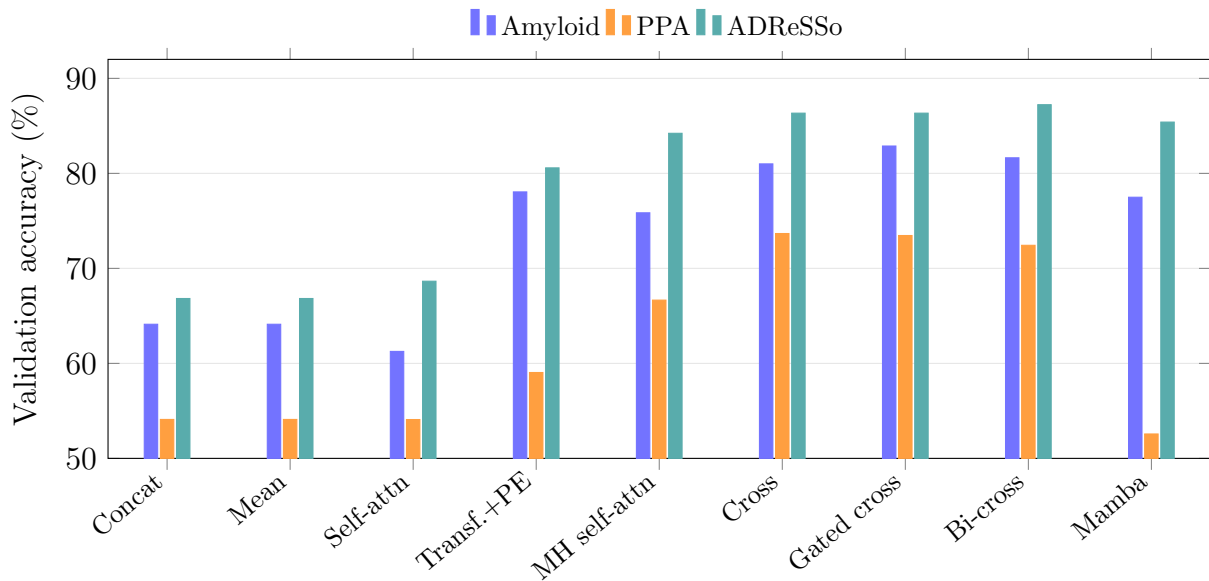
Figure 10: Validation accuracy of the fusion families on the three tasks (values from Table 8). The cross-attention family leads on every task, while Mamba’s drop to chance on PPA stands out as the clearest outlier.
