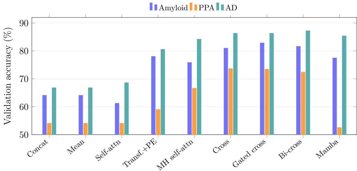
Figure 11: Validation accuracy of the fusion families on the three tasks (values from Table 10). The cross-attention family leads on every task, while Mamba’s drop to chance on PPA stands out as the clearest outlier. Abbreviations: Concat = concatenation, Mean = element-wise mean (both non-sequential baselines); Self-attn = self-attention, MH self-attn = multi-head self-attention, Transf.+PE = transformer with positional encoding; Cross = cross-attention, Gated cross = gated cross-attention, Bi-cross = bidirectional cross-attention; Mamba = selective state-space fusion.
