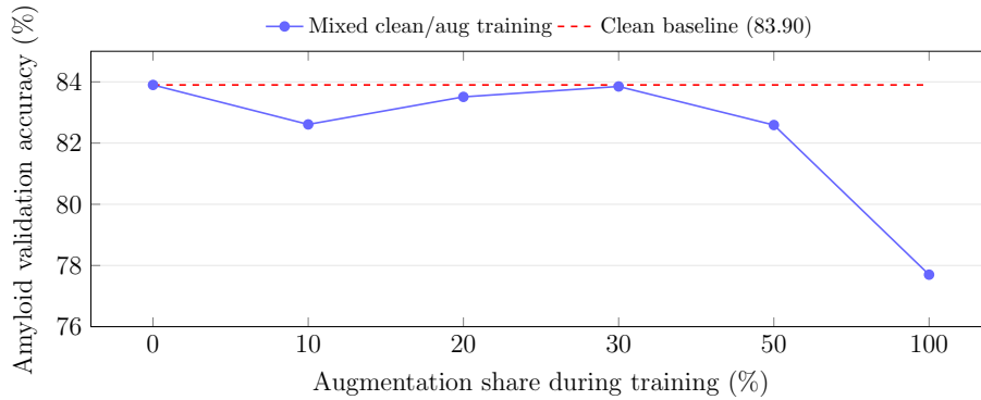
Figure 13: Amyloid validation accuracy as the training augmentation share p_{\text{aug}} increases ( res_model , bidirectional cross-attention, character token-to-token alignment, final layer, with handcrafted features). Accuracy stays near the clean baseline (dashed) under light mixing and drops sharply once augmentation dominates; the 30% share is the best setting and only matches, never beats, the clean baseline. Mean over seeds 43 and 3407, except the clean reference (seed 43).
