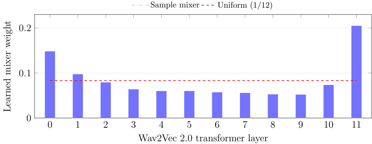
Figure 12: Learned per-layer weights of the per-utterance sample mixer on ADRessSo (seed 43, \tau = 0.1 , twelve Wav2Vec 2.0 layers). Weight concentrates on the uppermost layer (layer 11) and, secondarily, the lowest, both well above the uniform 1/12 baseline (dashed); the mean per-utterance spread of these weights is 0.24.
