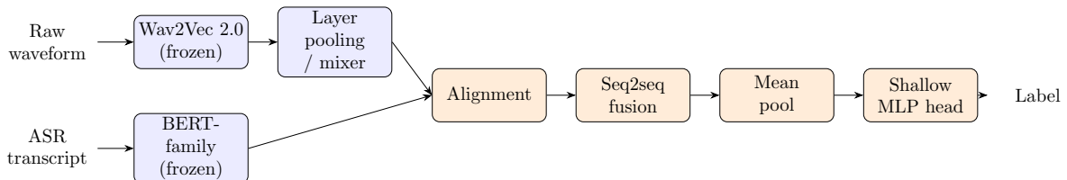
Figure 9: End-to-end architecture used in this thesis: frozen Wav2Vec 2.0 and BERT-family encoders (blue) produce acoustic and textual sequences, which are placed on a common index by the alignment step, combined by the trainable sequence-to-sequence fusion module (orange), and mapped to a task label by a shallow head. Blue blocks are frozen, orange blocks are trained.
