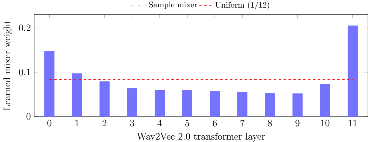
Figure 11: Learned per-layer weights of the per-utterance sample mixer on ADReSSo (seed 43, \tau = 0.1 , twelve Wav2Vec 2.0 layers). Weight concentrates on the uppermost layer (layer 11) and, secondarily, the lowest, both well above the uniform 1/12 baseline (dashed); the mean per-utterance spread of these weights is 0.24.
