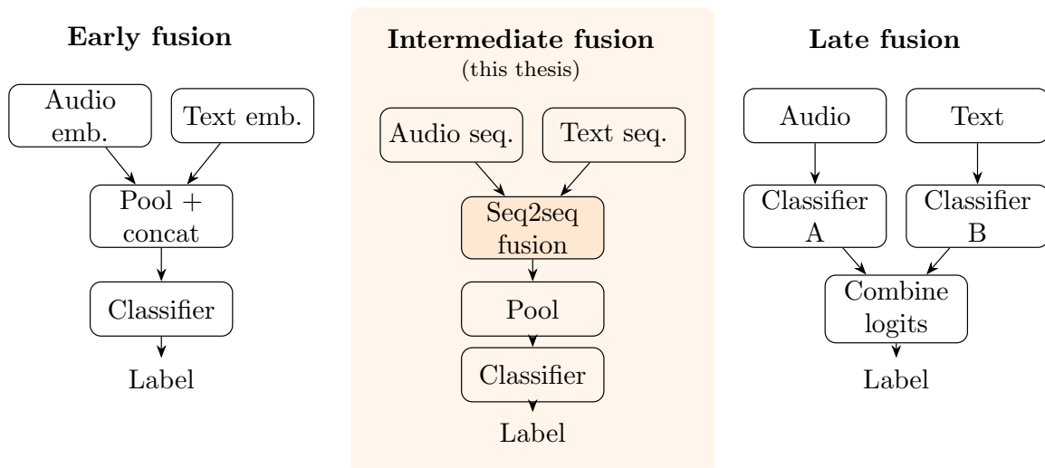
Figure 3: The three multimodal fusion paradigms. Early fusion pools and concatenates the modality embeddings into one vector before a single classifier; late fusion trains a classifier per modality and combines their outputs; intermediate fusion, the paradigm used in this thesis, processes both sequences jointly through a sequence-to-sequence module before pooling and classification.
