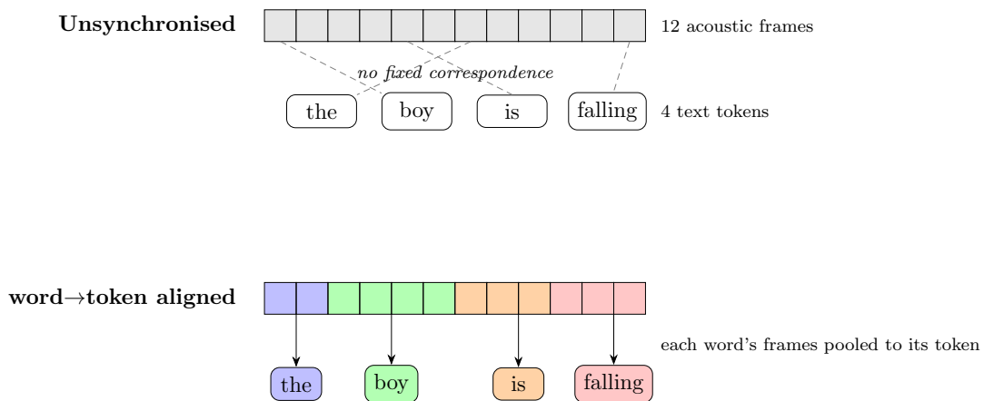
Figure 4: Cross-modal alignment between acoustic frames and text tokens, comparing unsynchronised input (top), where the two streams have no fixed correspondence, with word-to-token aligned input (bottom), where the frames spanned by each spoken word are pooled and attached to that word’s token.
