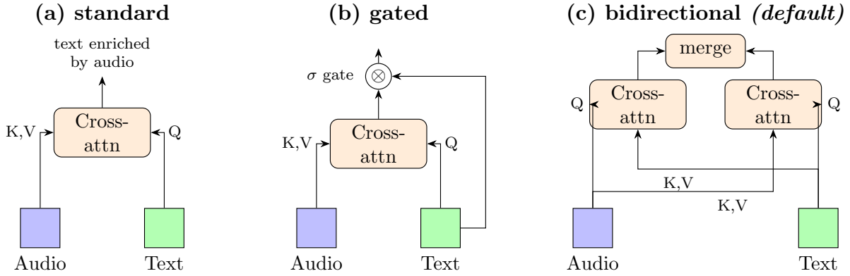
Figure 6: Cross-attention fusion variants: (a) standard, (b) gated, and (c) bidirectional.
