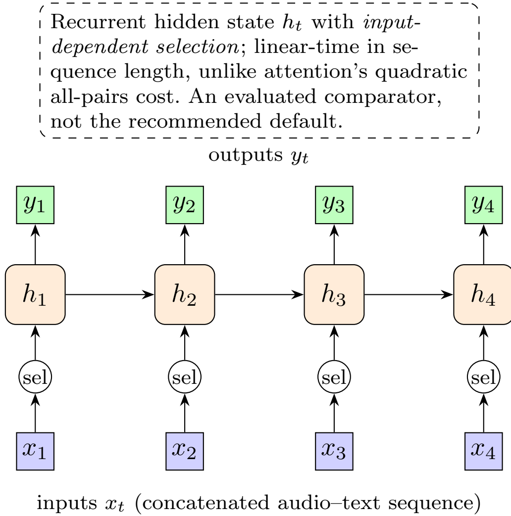
Figure 7: Mamba selective state-space fusion applied to the concatenated audio-text sequence.
