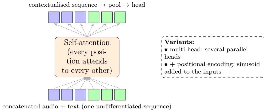
Figure 5: Self-attention fusion over the concatenated audio–text sequence.
