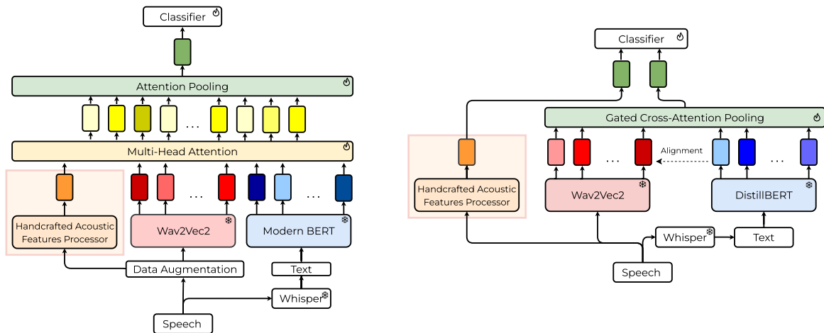
Figure 9: Architectural comparison of the two multimodal frameworks this thesis builds on. The left panel shows the Double Multi-Head Attention Multimodal (DMHAM) system; the right panel shows the CogniAlign framework. They share a two-stream skeleton but differ in their encoders, ASR, and alignment: CogniAlign aligns acoustic frames to subword tokens, whereas DMHAM fuses segment-level representations.
