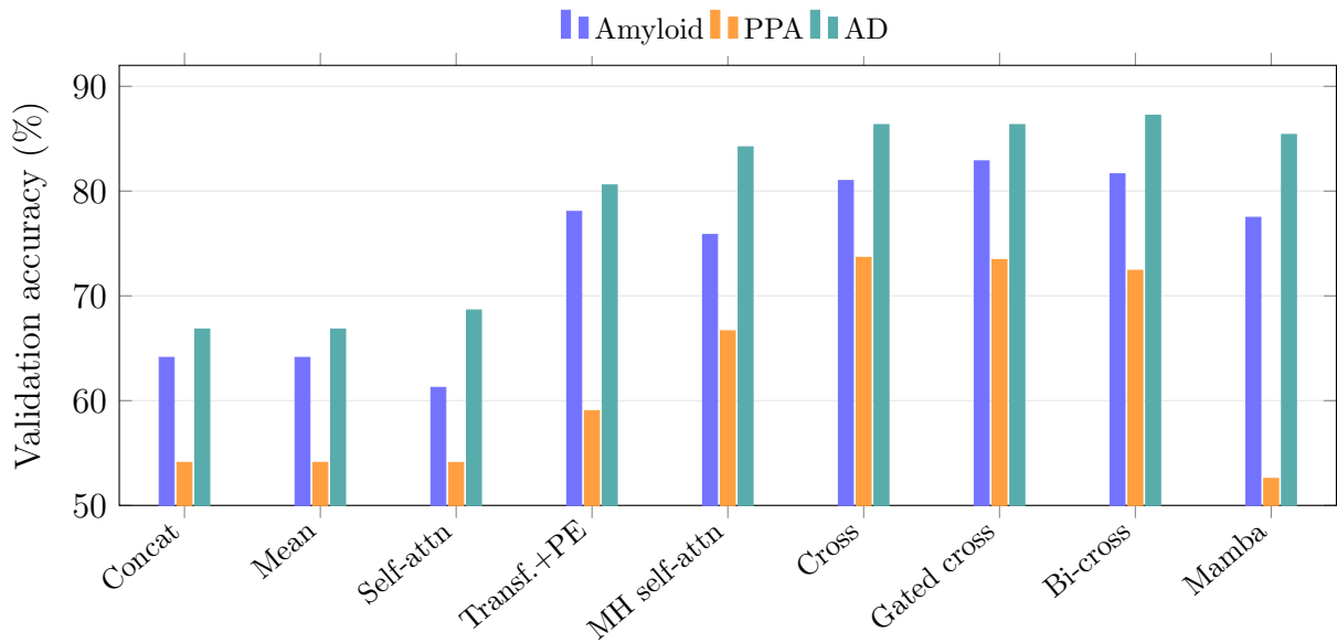
Figure 10: Validation accuracy of the fusion families on the three tasks (values from Table 9). The cross-attention family leads on every task, while Mamba’s drop to chance on PPA stands out as the clearest outlier. Abbreviations: Concat = concatenation, Mean = element-wise mean (both non-sequential baselines); Self-attn = self-attention, MH self-attn = multi-head self-attention, Transf.+PE = transformer with positional encoding; Cross = cross-attention, Gated cross = gated cross-attention, Bi-cross = bidirectional cross-attention; Mamba = selective state-space fusion.
