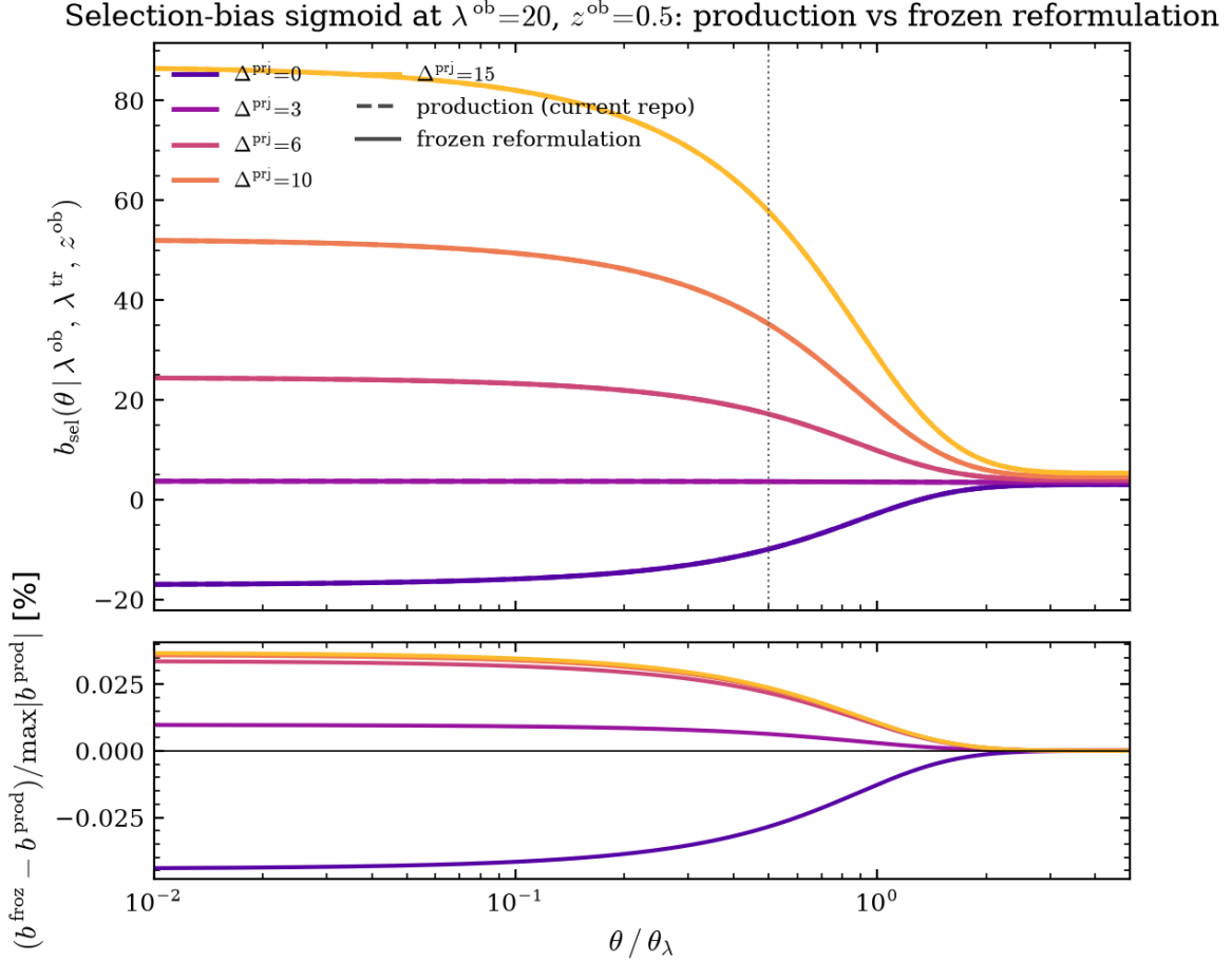
Figure 4: b_{\text{sel}}(\theta \mid \lambda^{\text{ob}}, \lambda^{\text{tr}}, z^{\text{ob}}) at (\lambda^{\text{ob}}, z^{\text{ob}}) = (20, 0.5) for \Delta^{\text{prj}} \in \{0, 3, 6, 10, 15\} : production (dashed) vs frozen (solid, visually coincident). Bottom : residual normalised by \max_{\theta} |b^{\text{prod}}| per \Delta^{\text{prj}} ; worst 0.044% at \Delta^{\text{prj}} = 0 .
