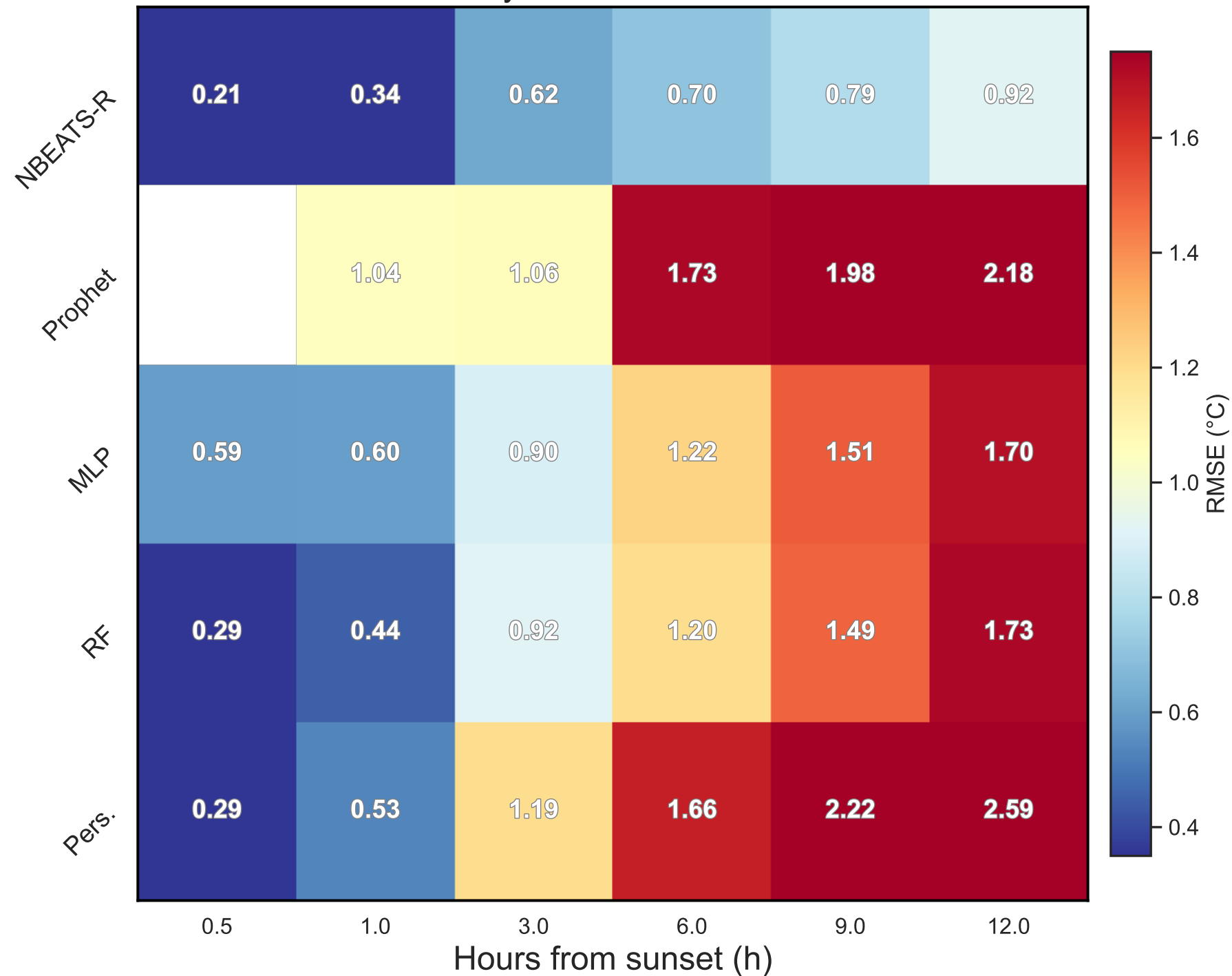
RMSE by Model and Lead Time
