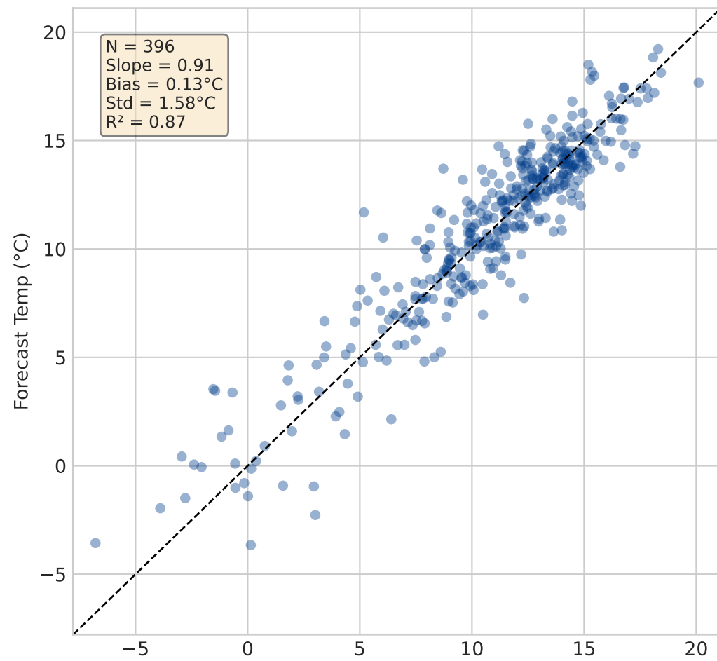
NBEATSx-Blend (12h)
