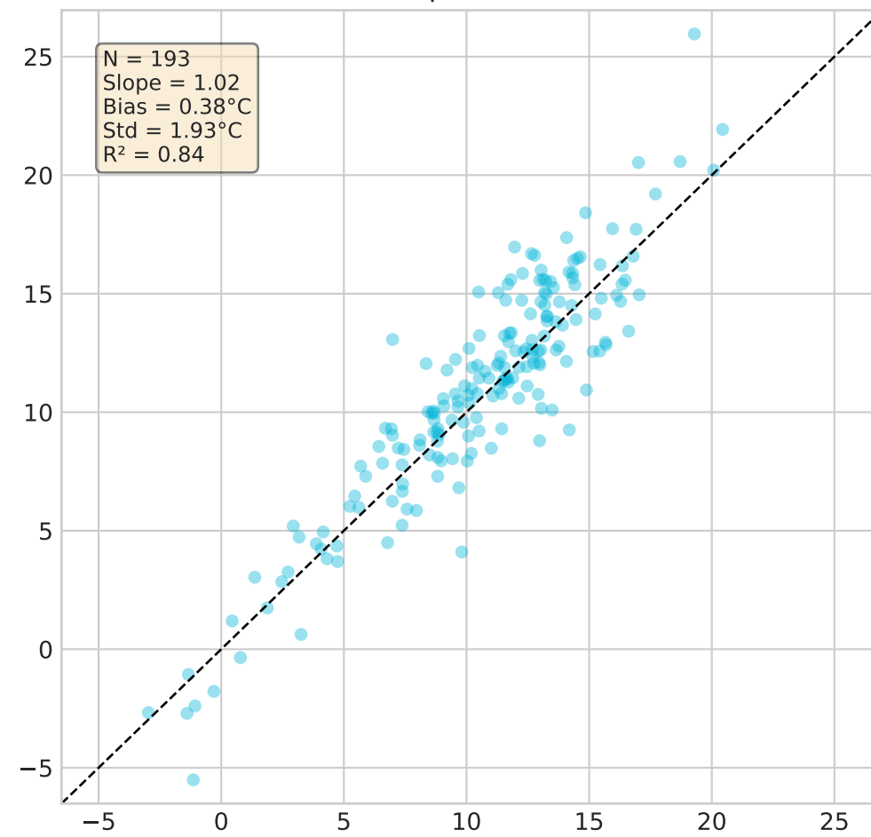
Prophet (6h)
