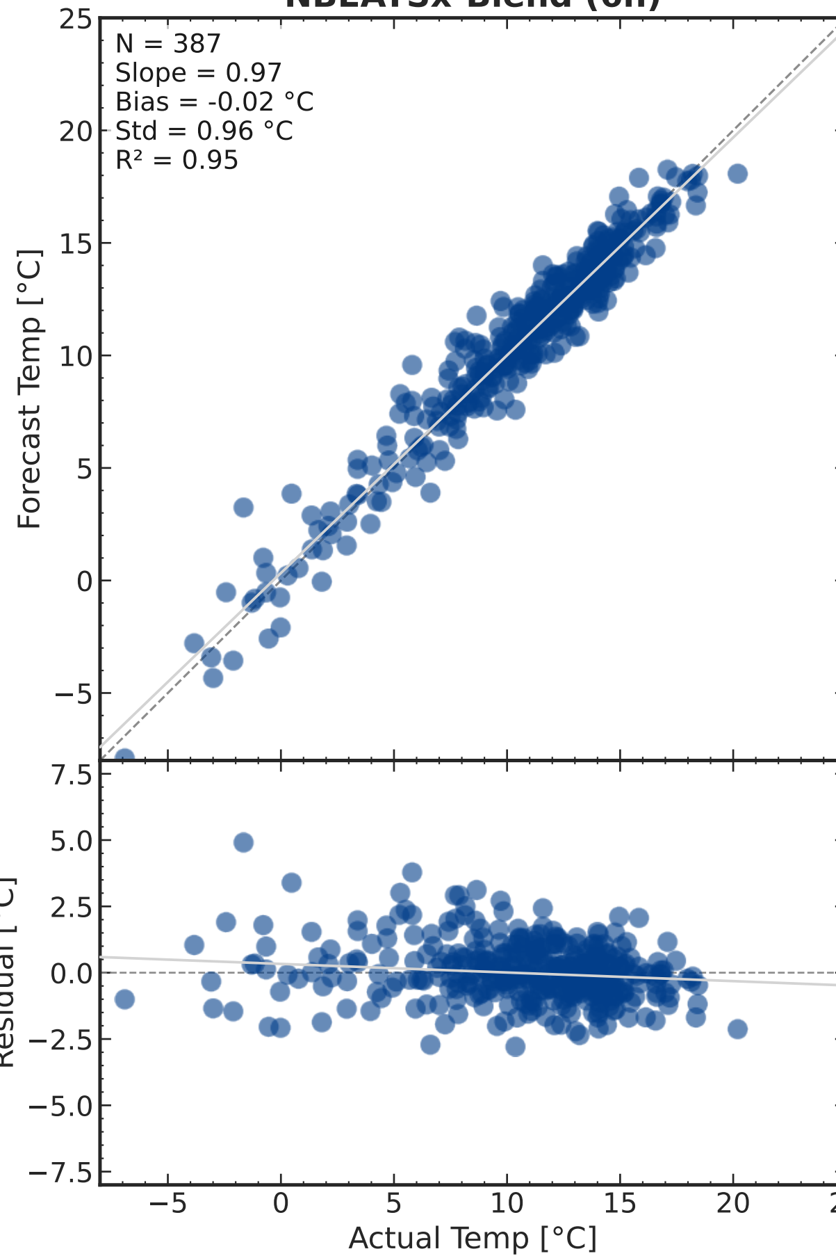
NBEATSx-Blend (6h)
