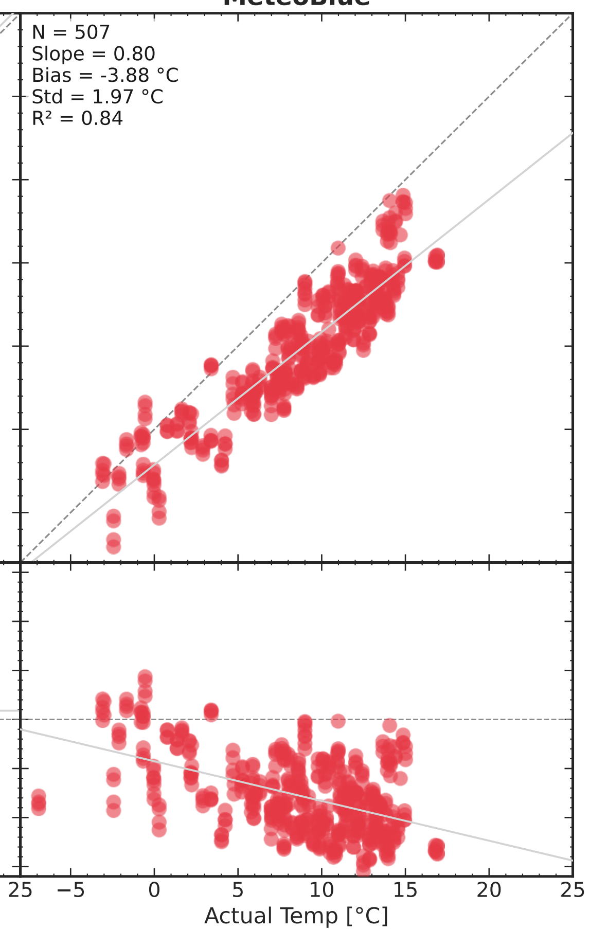
MeteoBlue
