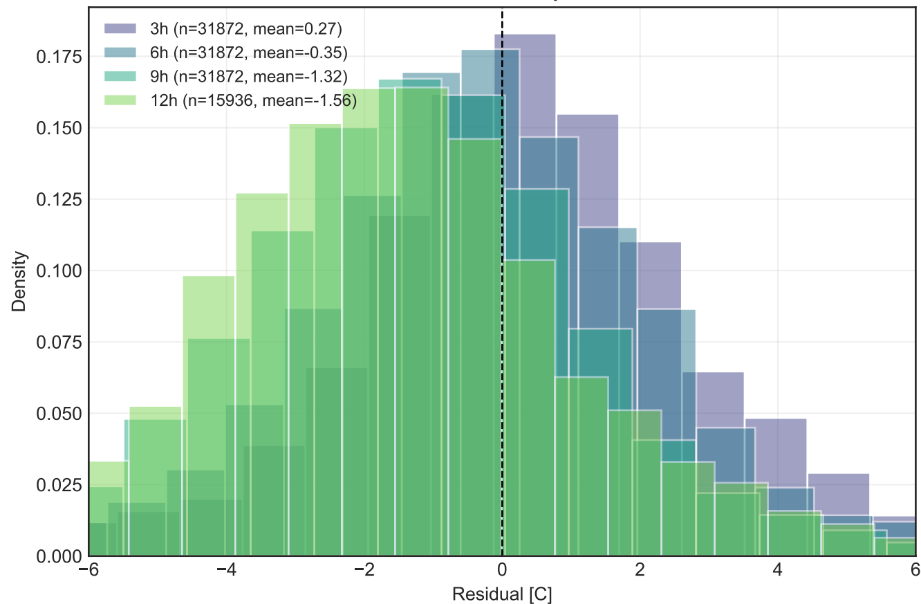
Residual Distribution by Lead Time
