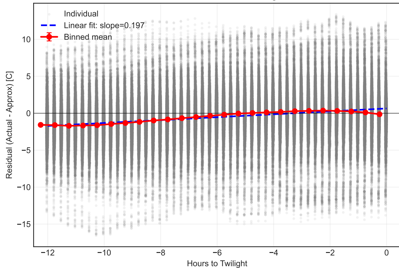
NBEATSx Residual Pattern Before Ridge Correction
