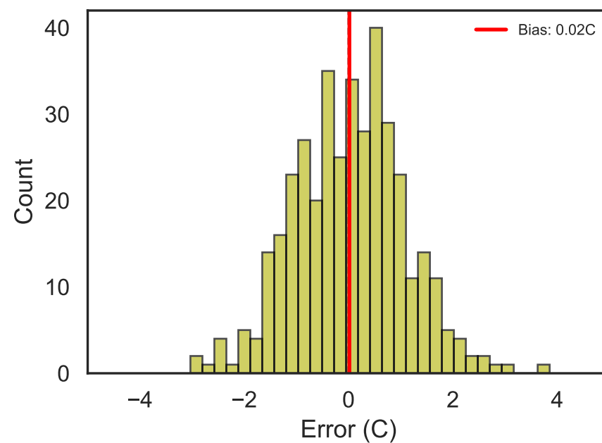
MLP RMSE: 1.06C
