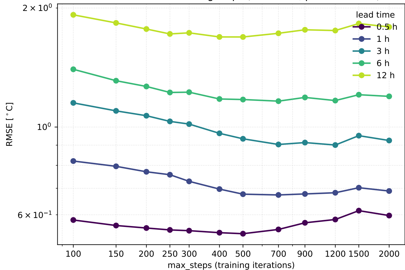
NBEATSx RMSE vs training steps (width=16, pre-2025 train)
