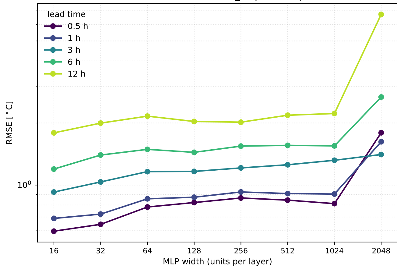
NBEATSx RMSE vs MLP width (max_steps=200, pre-2025 train)
