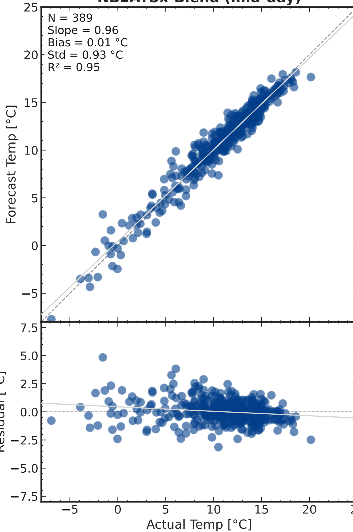
NBEATSx-Blend (mid-day)
