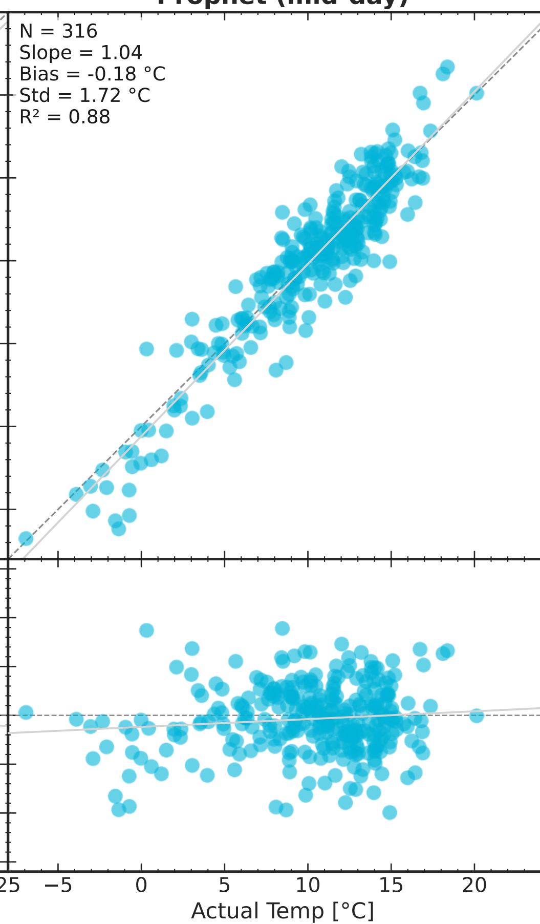
Prophet (mid-day)
