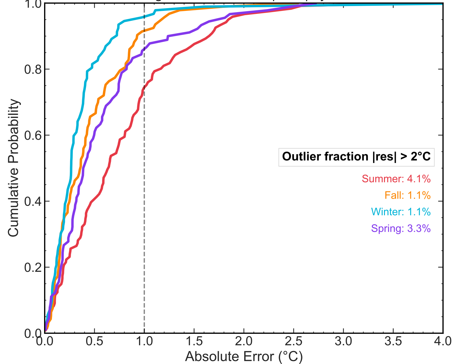
Morning forecast: CDF of |error| by season
