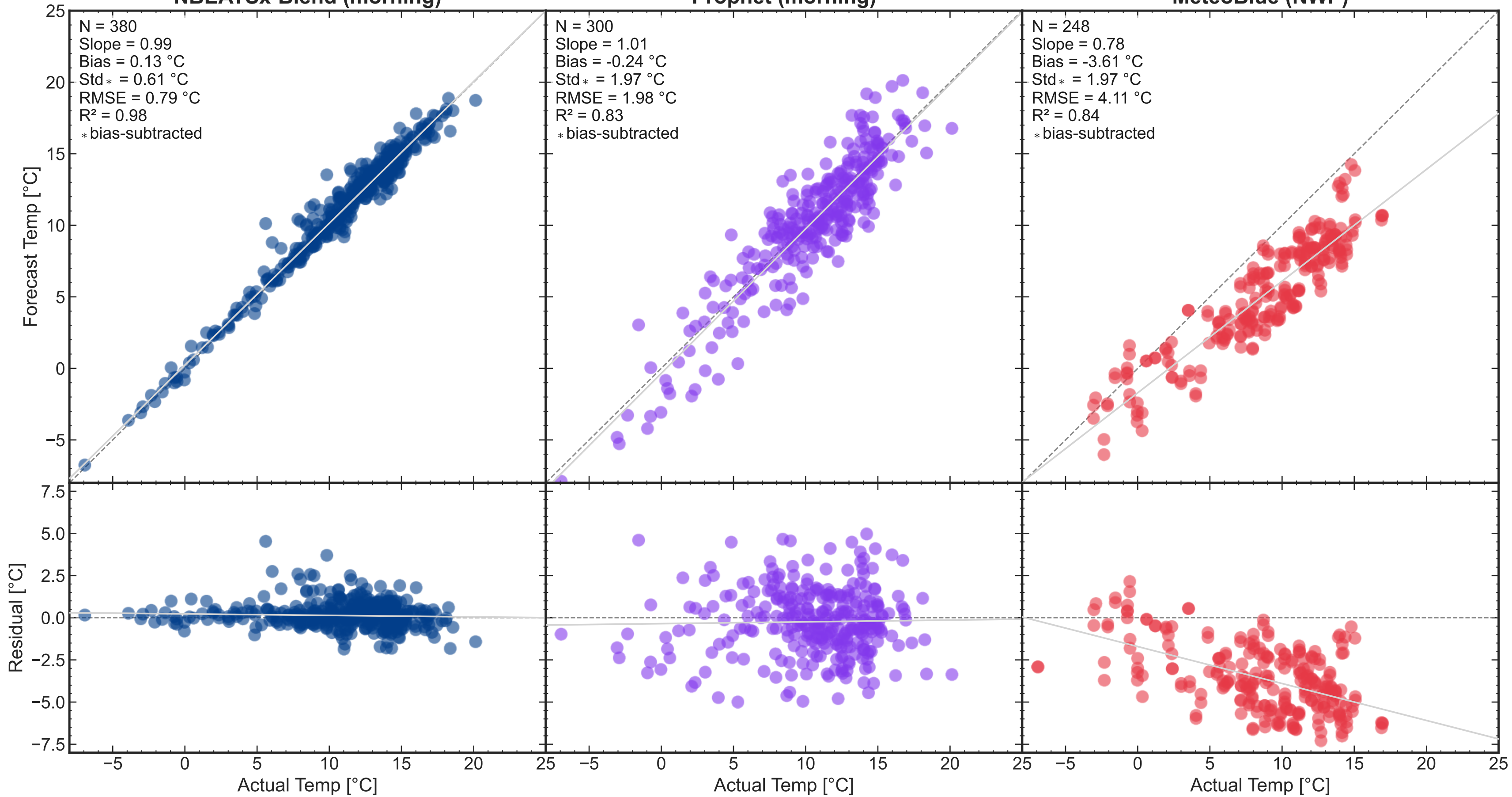
NBEATSx-Blend (morning)
