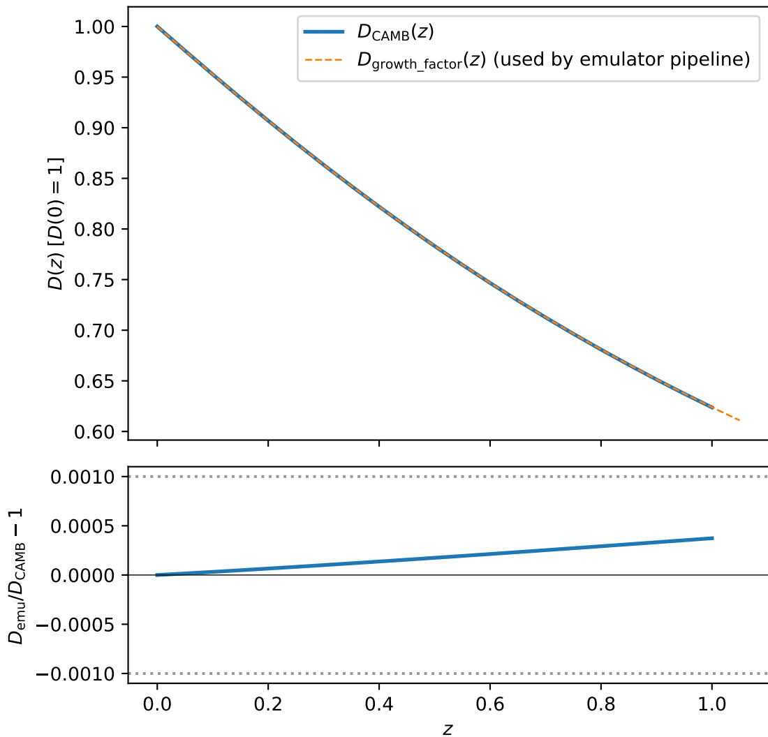
Growth factor used to rescale P(k, z = 0) \rightarrow P(k, z)
