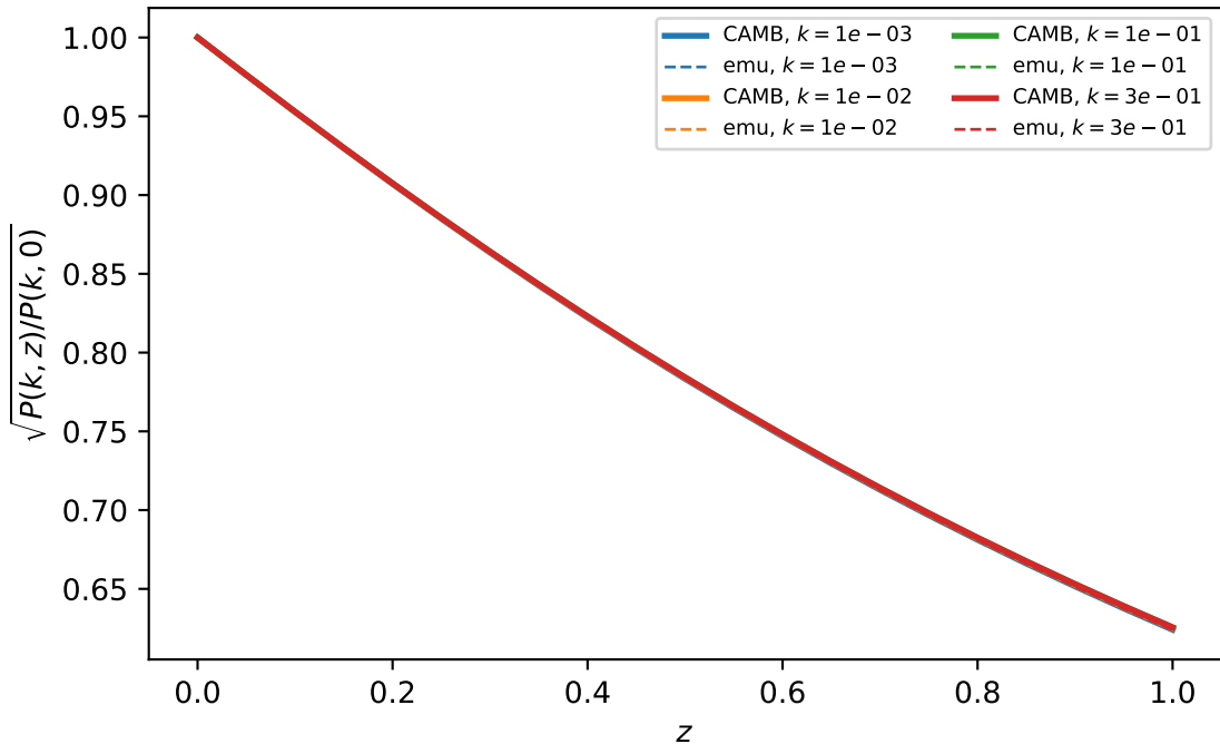
Effective D(k, z) from P_{\text{cb}} : CAMB vs emulator
