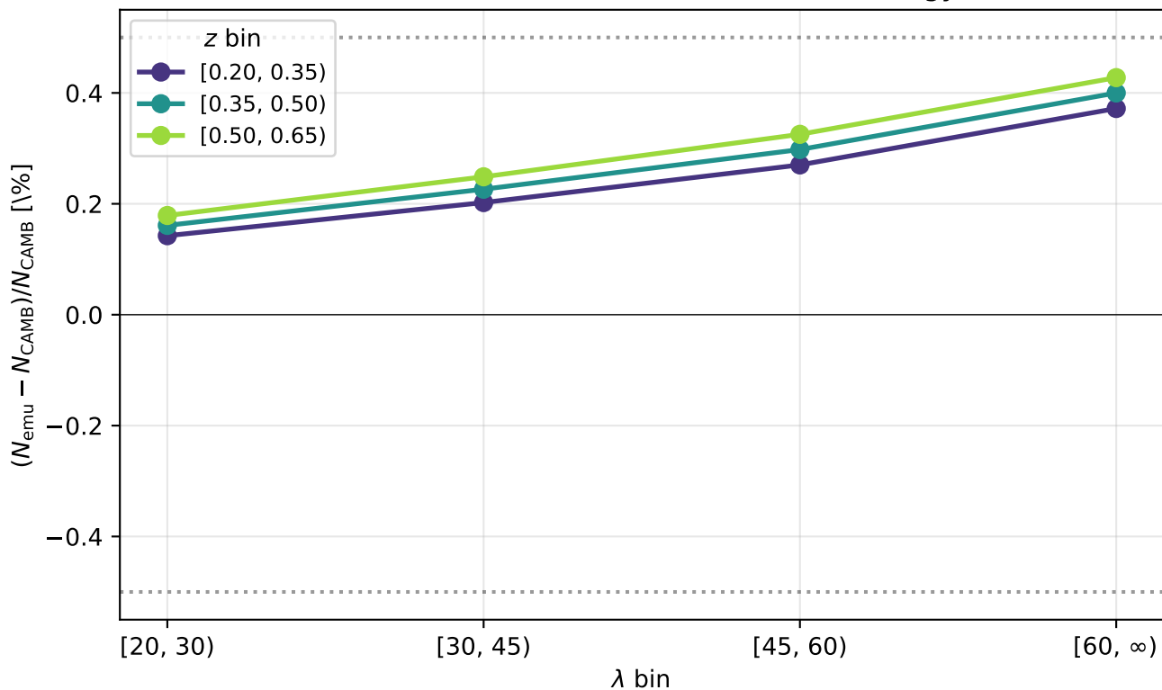
Number-counts residual at the fiducial cosmology (v2c)
