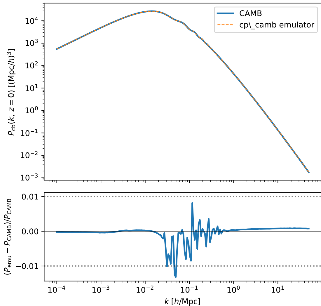
CDM+baryon linear P(k, z=0)
