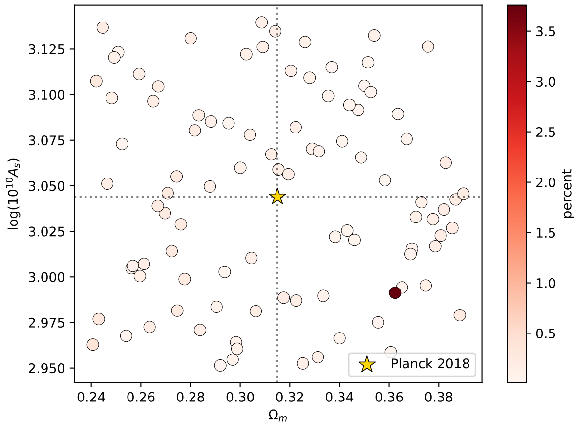
Mean |\Delta N/N| over 12 (\lambda, z) bins [%]
