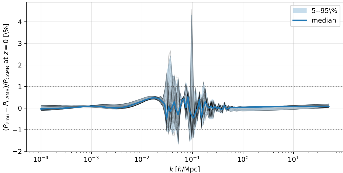
Planck-centered scan: P_{\text{cb}}(k, z = 0) emulator error
