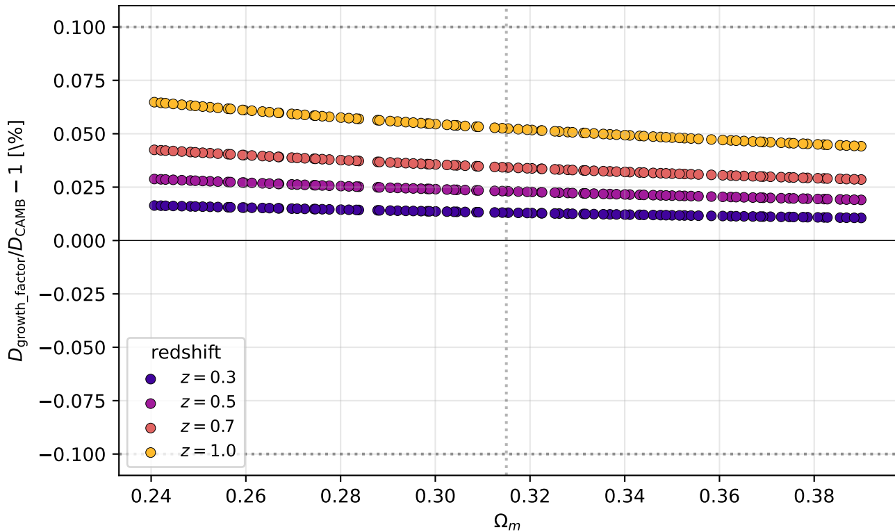
Growth-factor residual vs \Omega_m (v2c Planck scan)
