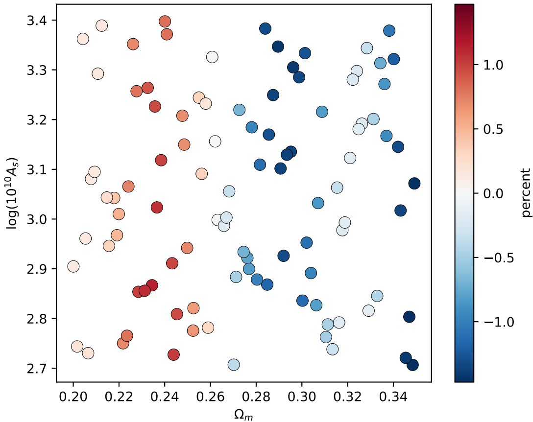
\Delta P/P at k = 0.096 \, h/\text{Mpc} , z = 0 [\%]
