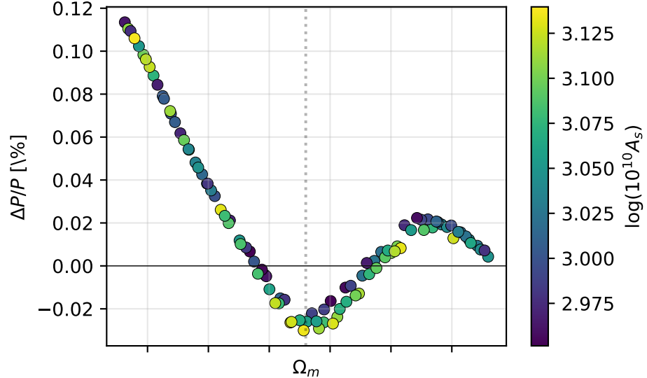
v2c: emulator P(k, z = 0) error vs \Omega_m (Planck scan)
