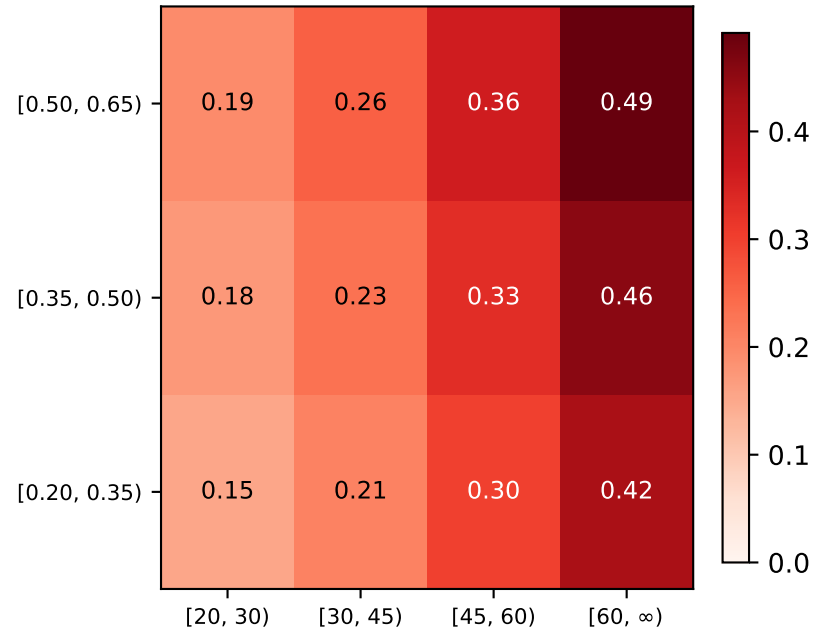
|\Delta N/N|_{\text{max}} over 97 samples [%]
