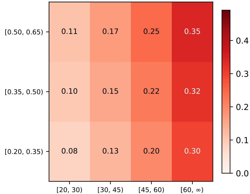
|\Delta N/N|_{\text{median}} over 97 samples [%]
