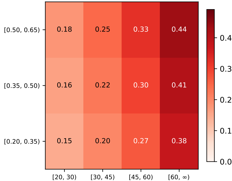
|\Delta N/N|_{\text{p95}} over 97 samples [%]
