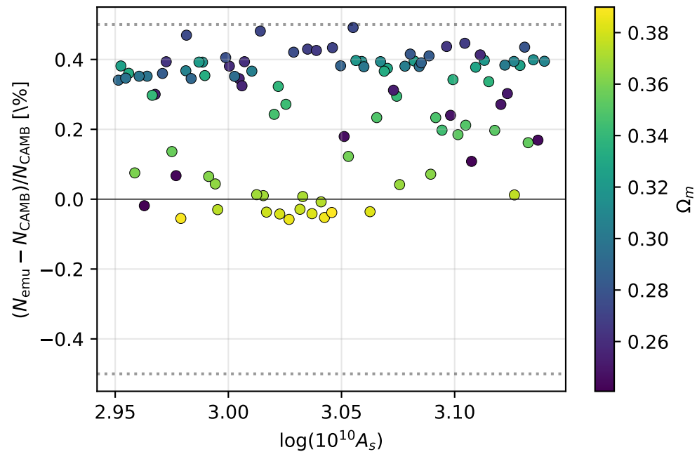
v2c: residual vs cosmology (worst bin: z[0.50, 0.65) , \lambda[60, \infty) )
