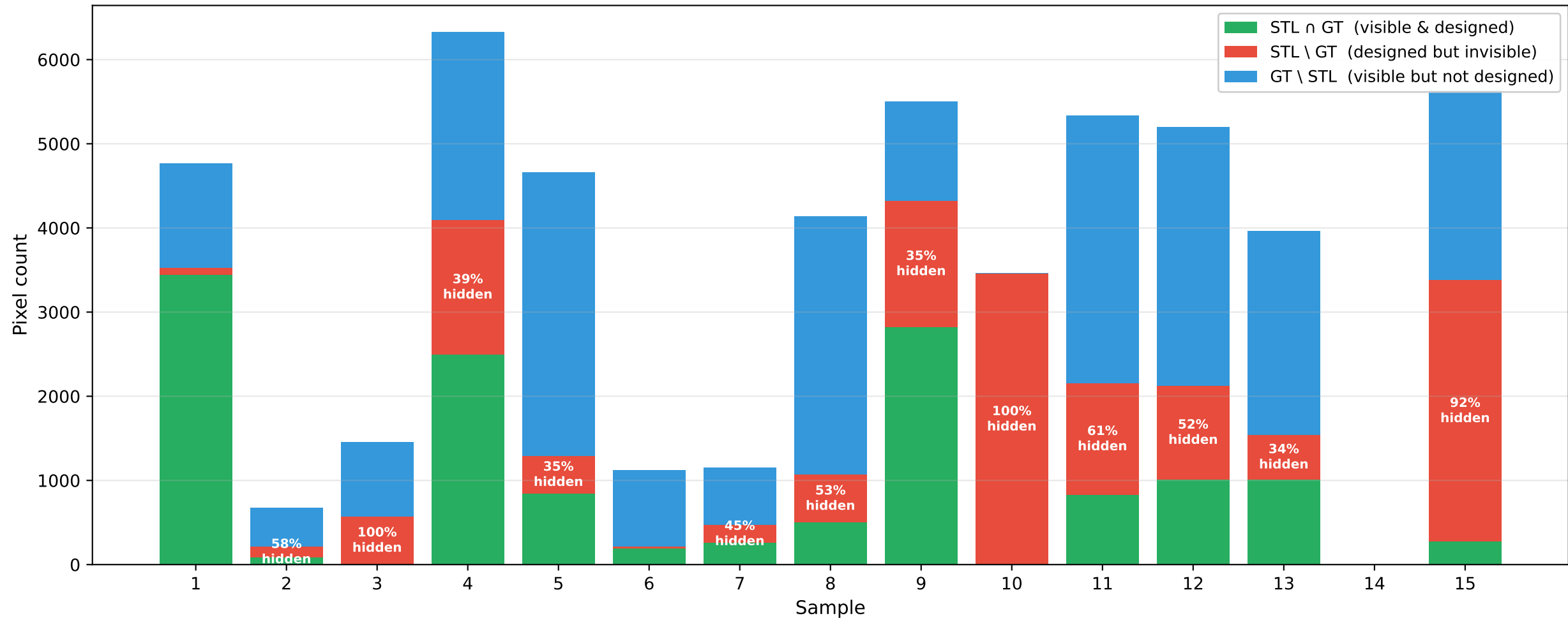
Designed (STL) vs detectable (manual GT) void area per sample
