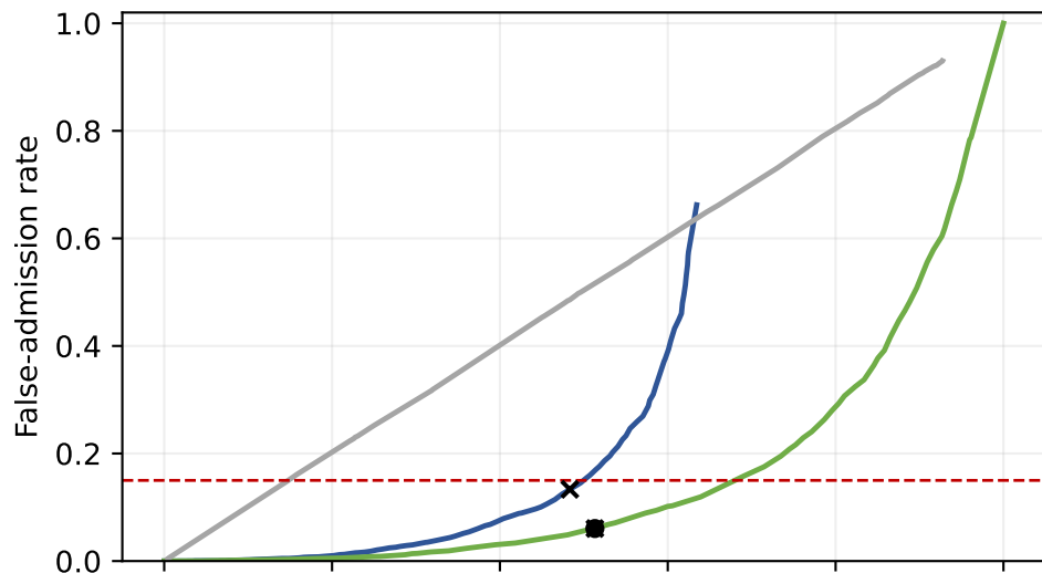
CVEfixes: false admission curve
