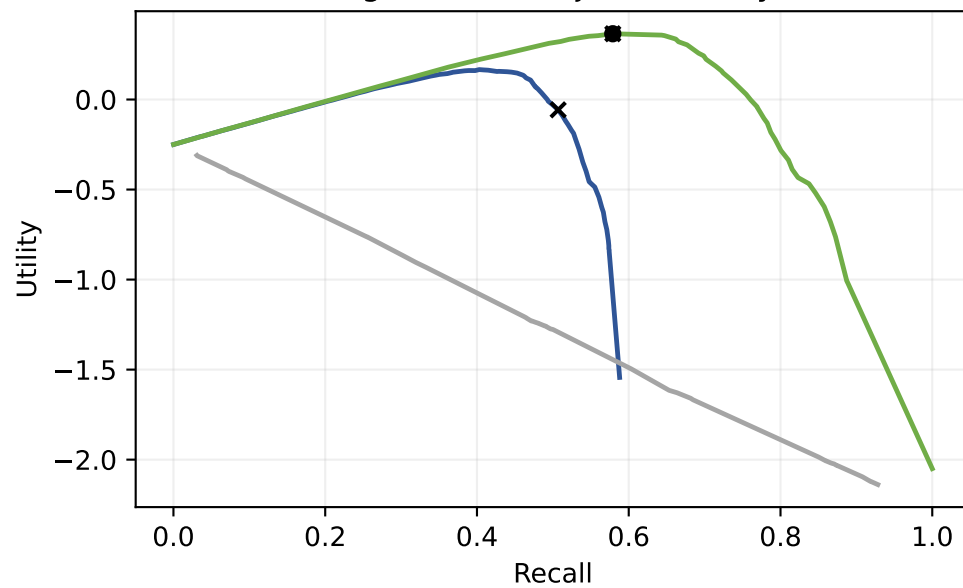
BigVul: debt-adjusted utility
