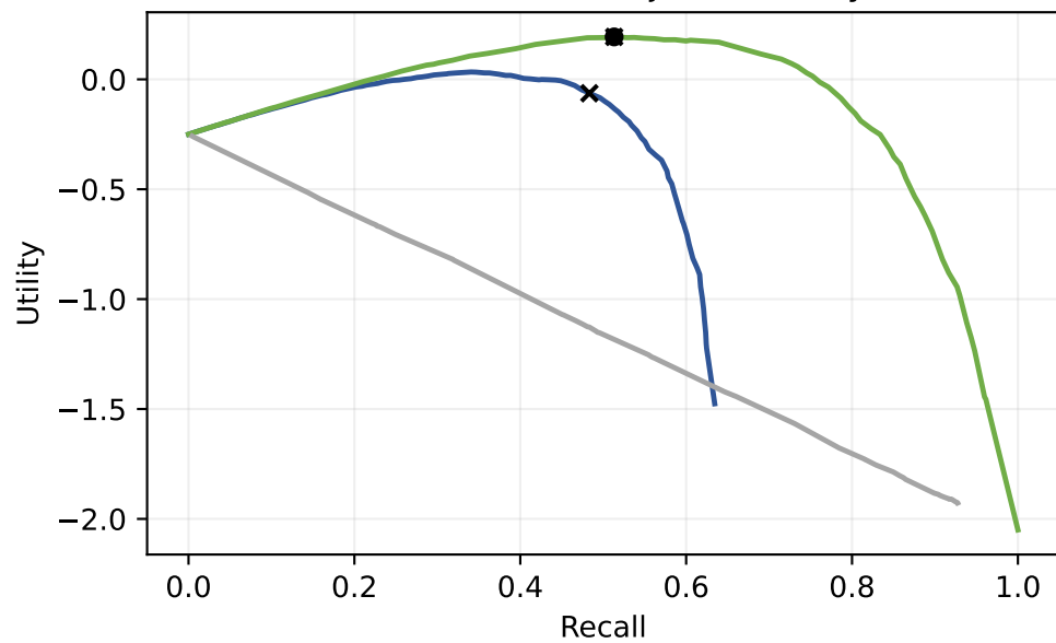
CVEfixes: debt-adjusted utility
