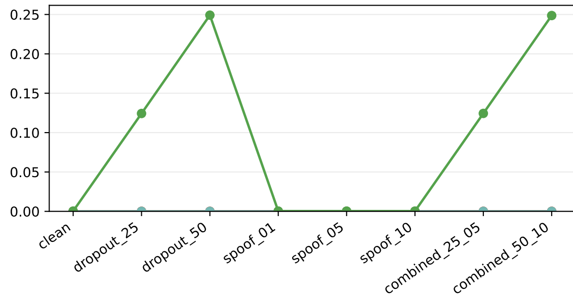
Abstain / validation-debt rate
