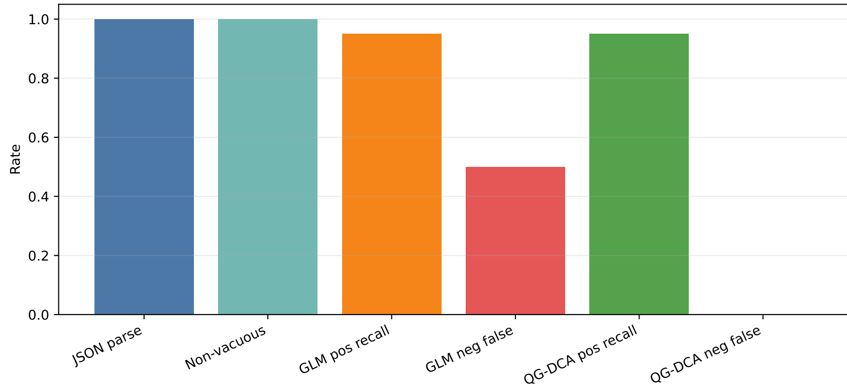
LXXXVI GLM candidate-oracle calibration
