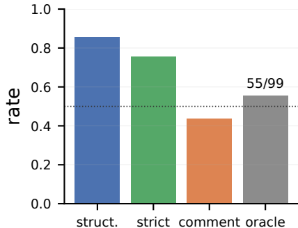
(b) ASR admission contraction
